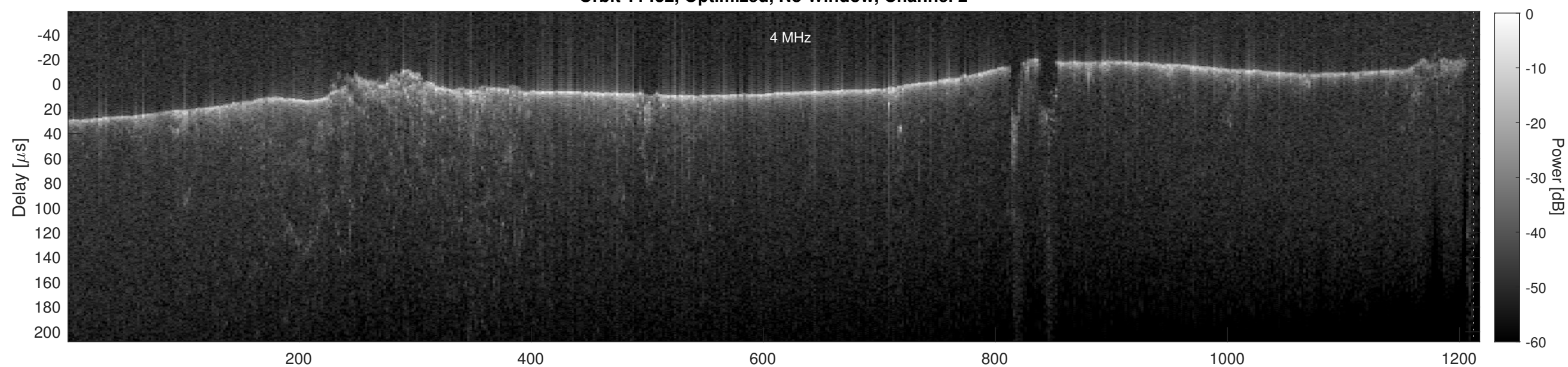
Orbit 11432, Cluttergram
