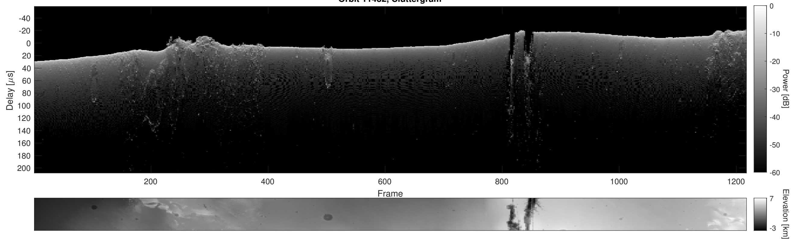
Orbit 11432, Cluttergram
