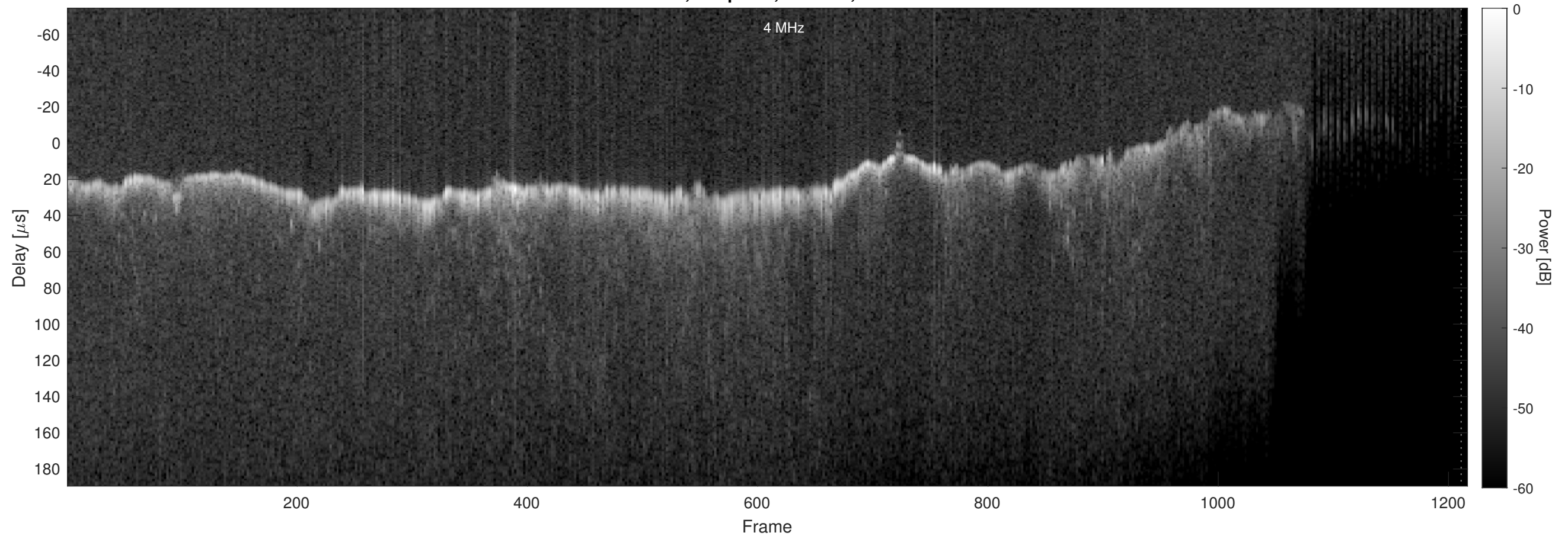
Orbit 11433, Chapman, Window, Channel 2
