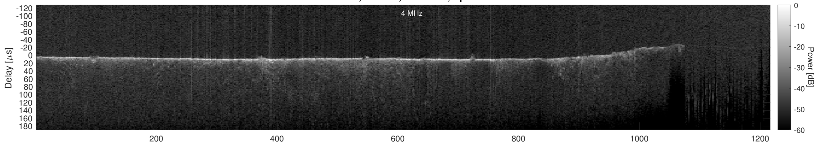
Orbit 11433, Cluttergram
