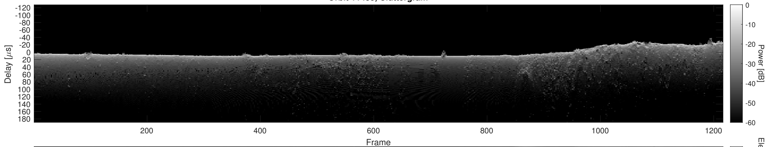
Orbit 11433, Cluttergram
