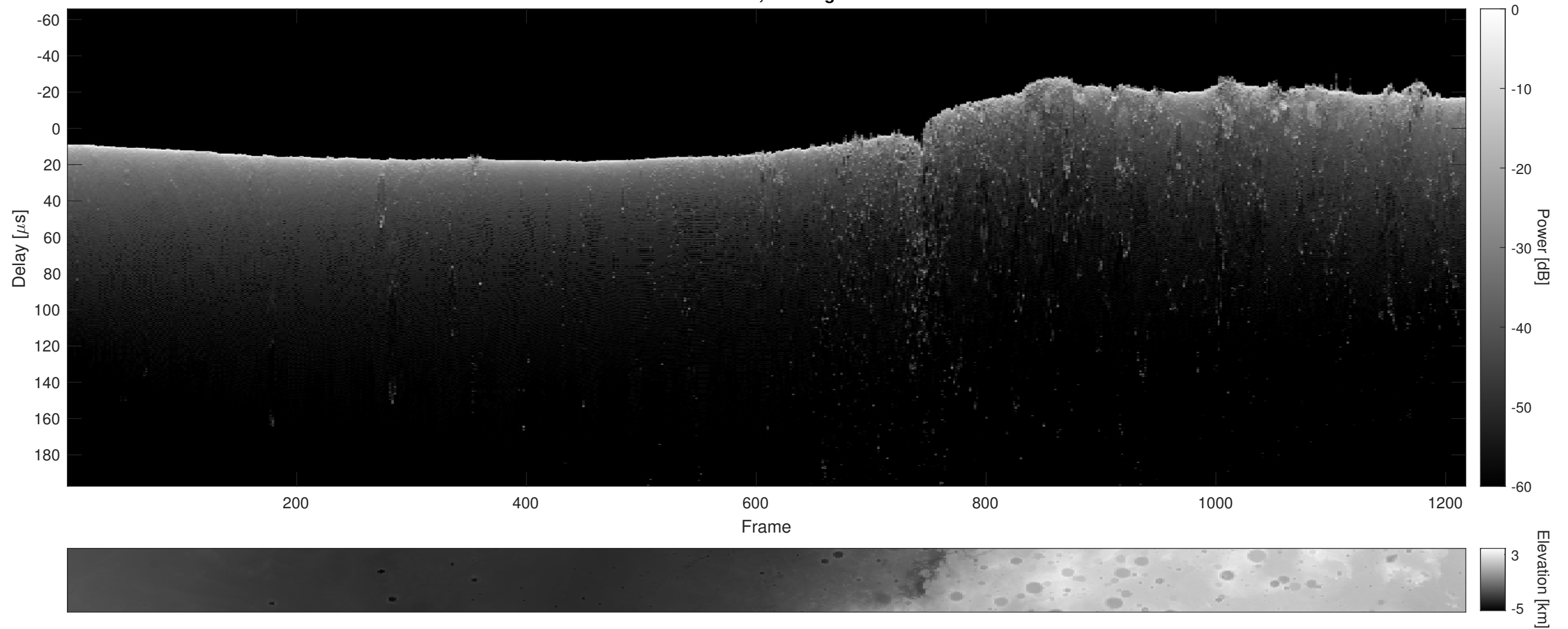
Orbit 11437, Cluttergram
