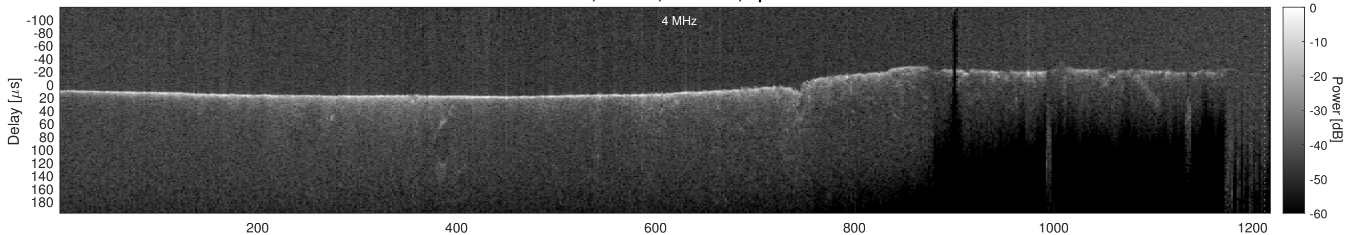
Orbit 11437, Cluttergram
