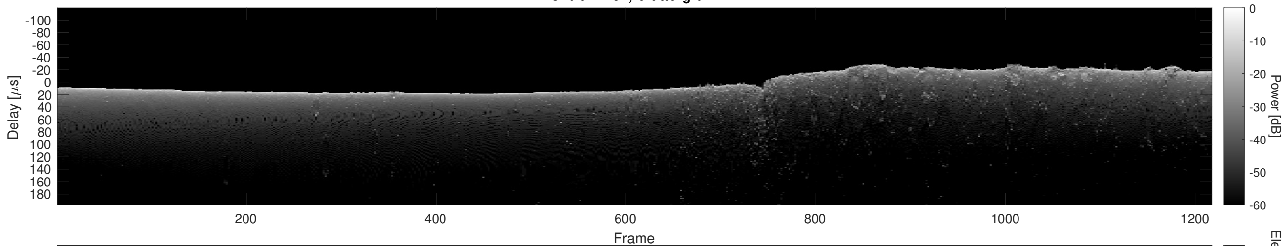
Orbit 11437, Cluttergram
