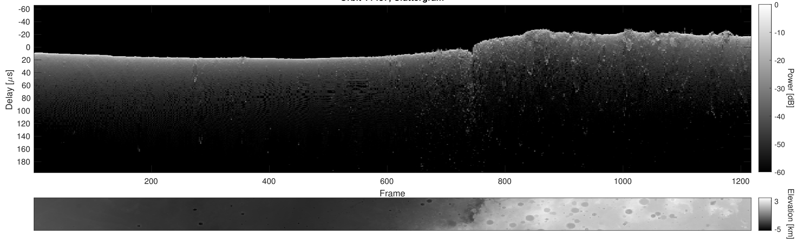
Orbit 11437, Cluttergram
