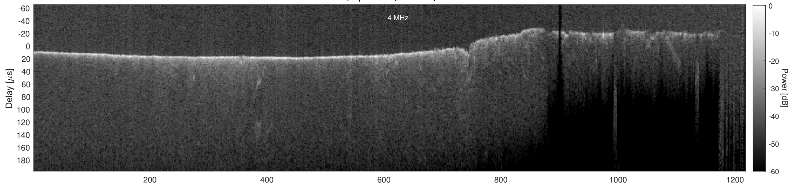
Orbit 11437, Cluttergram
