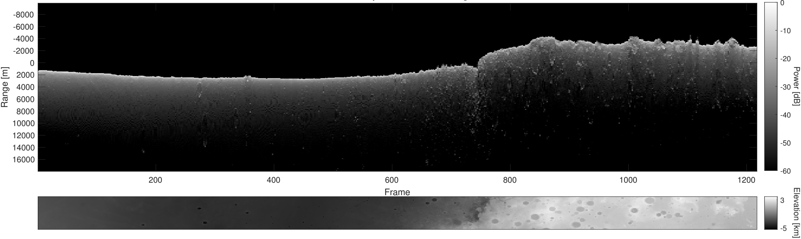
Orbit 11437, Depth-Corrected Cluttergram
