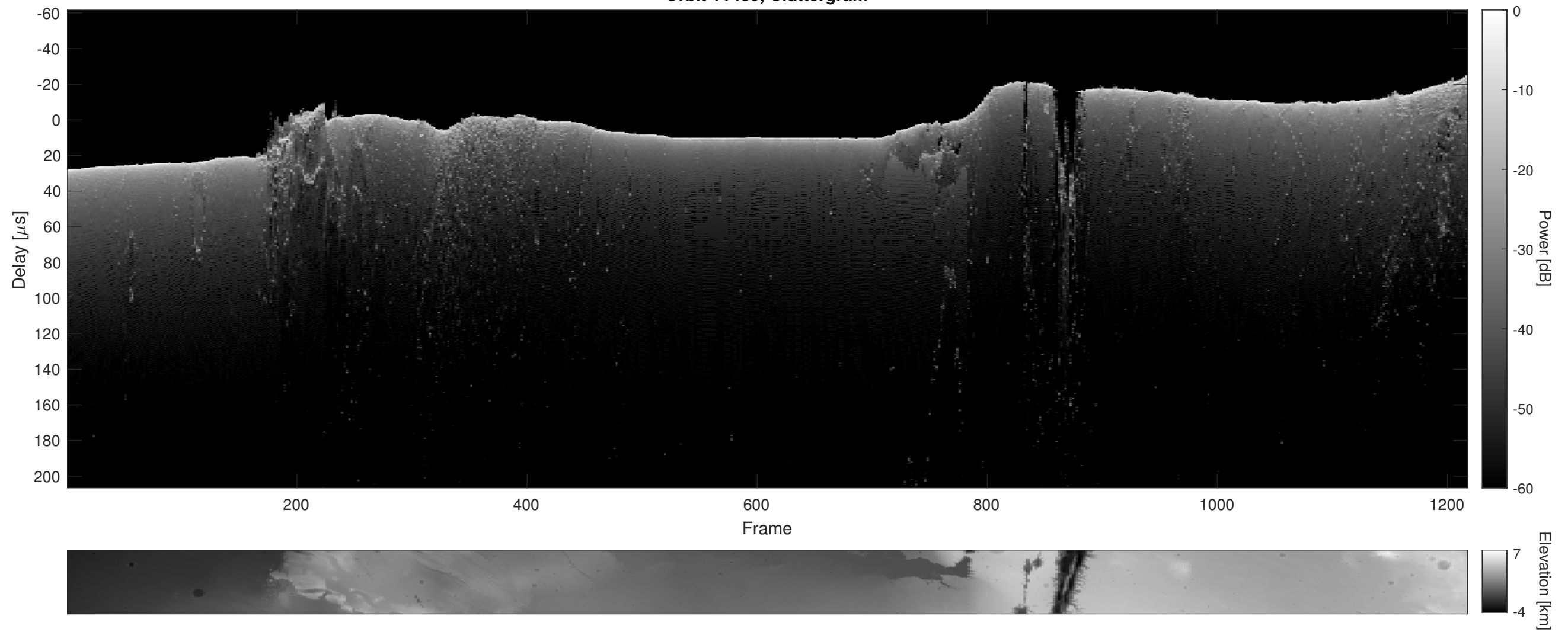
Orbit 11439, Cluttergram
