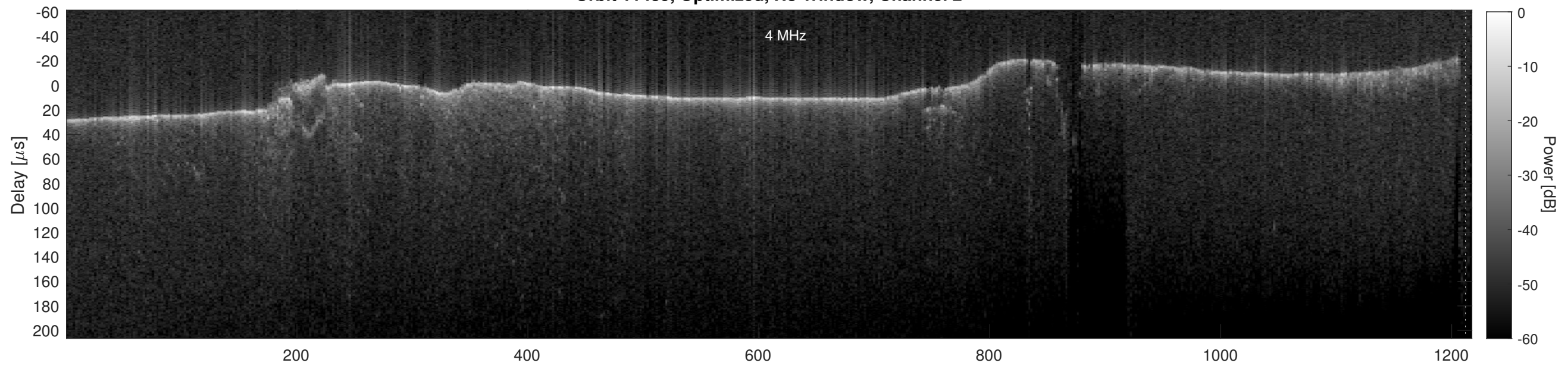
Orbit 11439, Cluttergram
