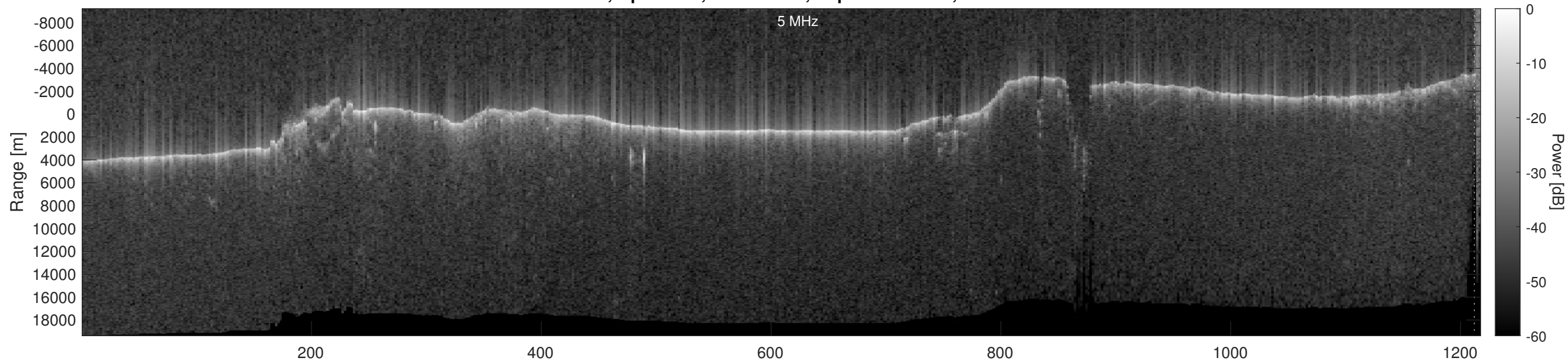
Orbit 11439, Optimized, No Window, Depth-Corrected, Channel 2
