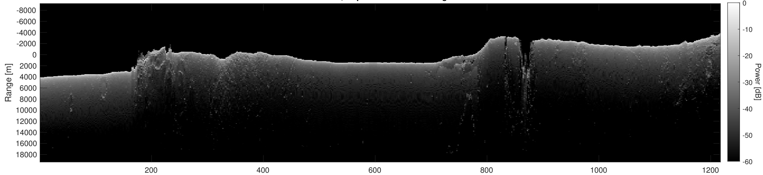
Orbit 11439, Depth-Corrected Cluttergram
