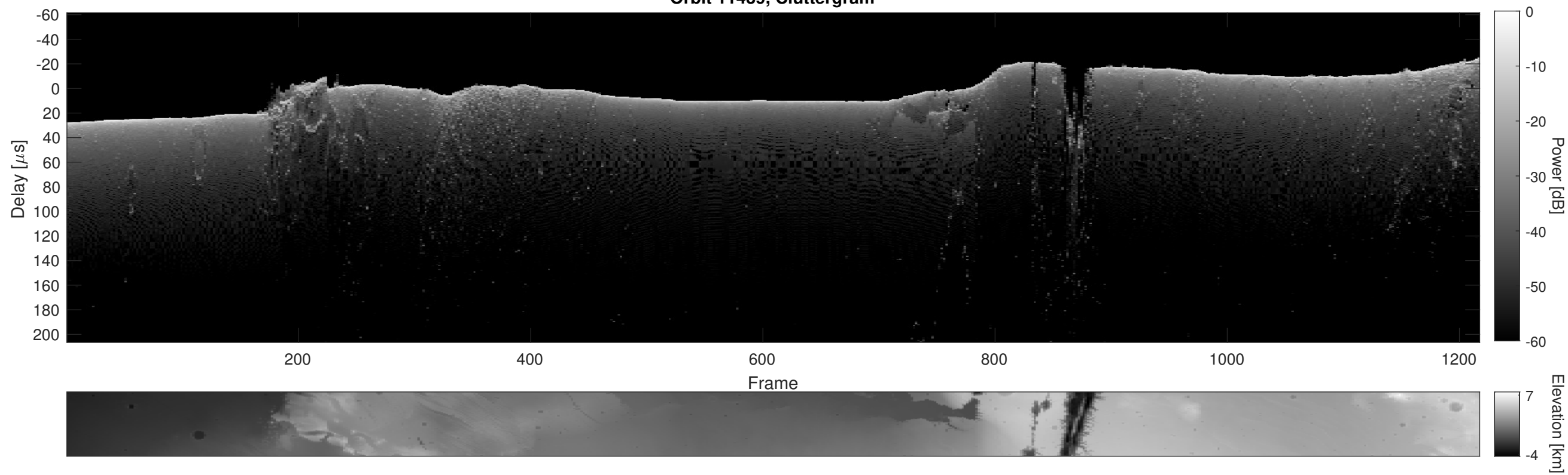
Orbit 11439, Cluttergram
