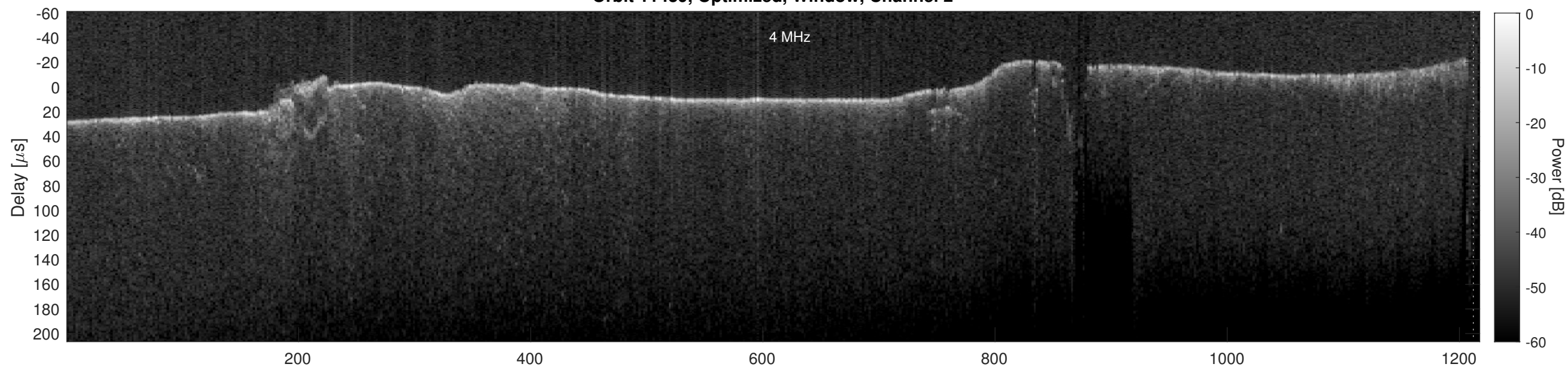
Orbit 11439, Cluttergram
