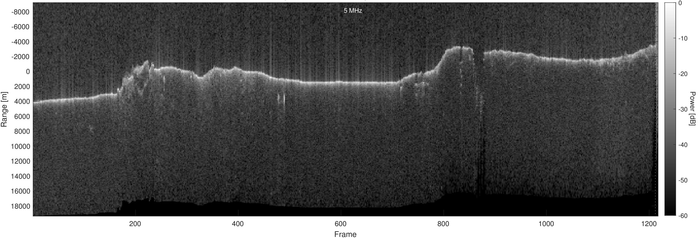
Orbit 11439, Optimized, Window, Depth-Corrected, Channel 2
