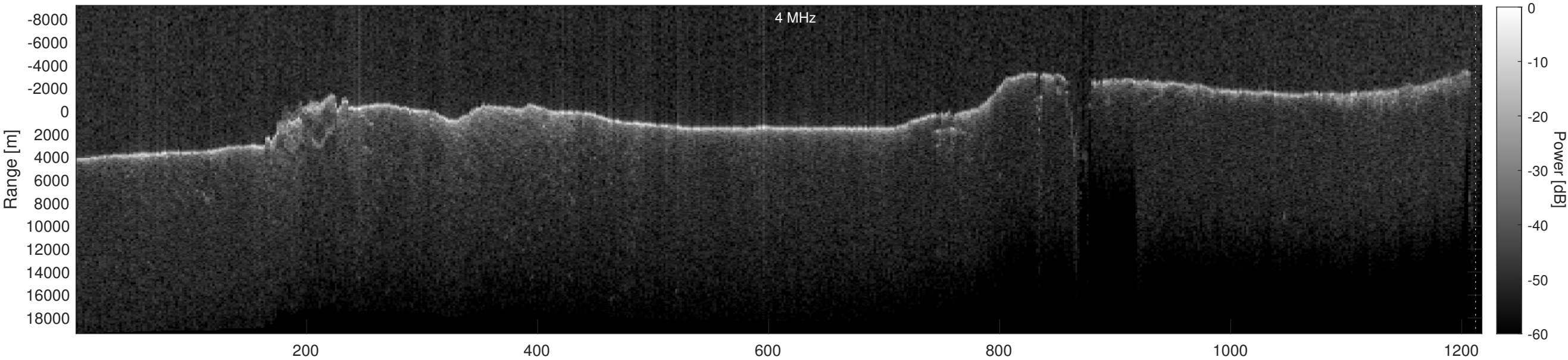
Orbit 11439, Depth-Corrected Cluttergram
