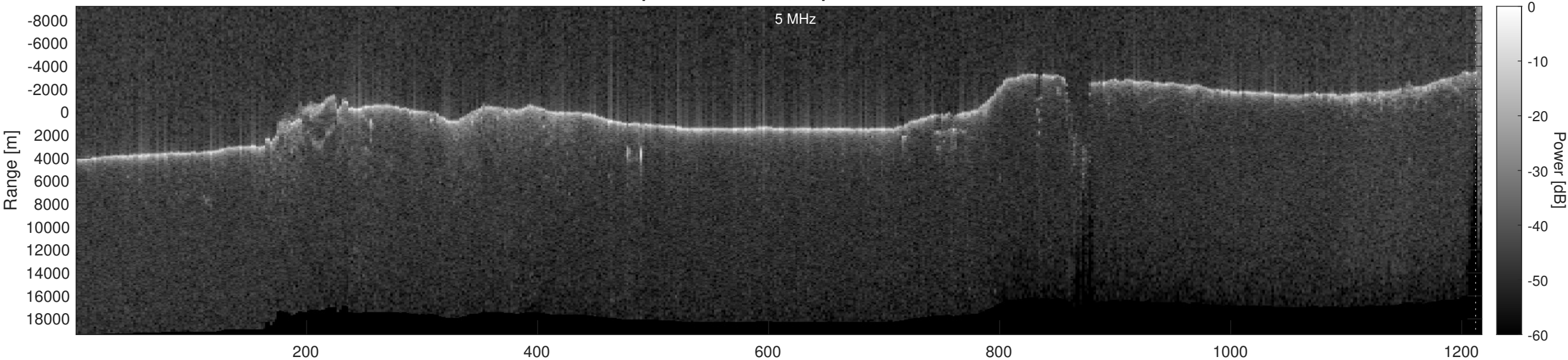
Orbit 11439, Optimized, Window, Depth-Corrected, Channel 2
