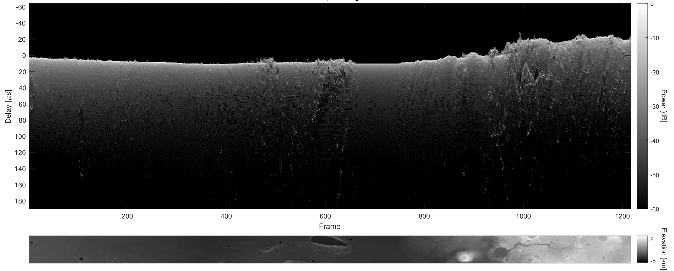
Orbit 11440, Cluttergram
