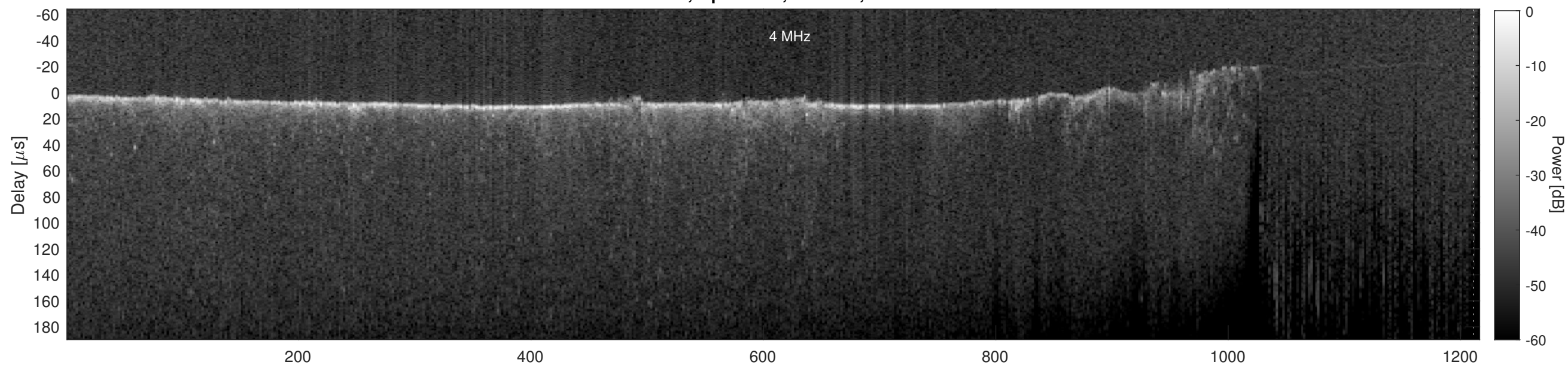
Orbit 11440, Cluttergram
