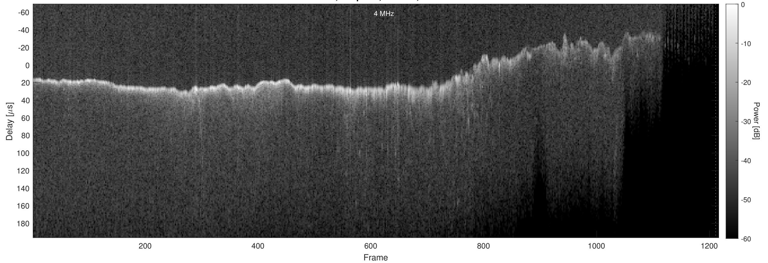
Orbit 11444, Chapman, Window, Channel 2
