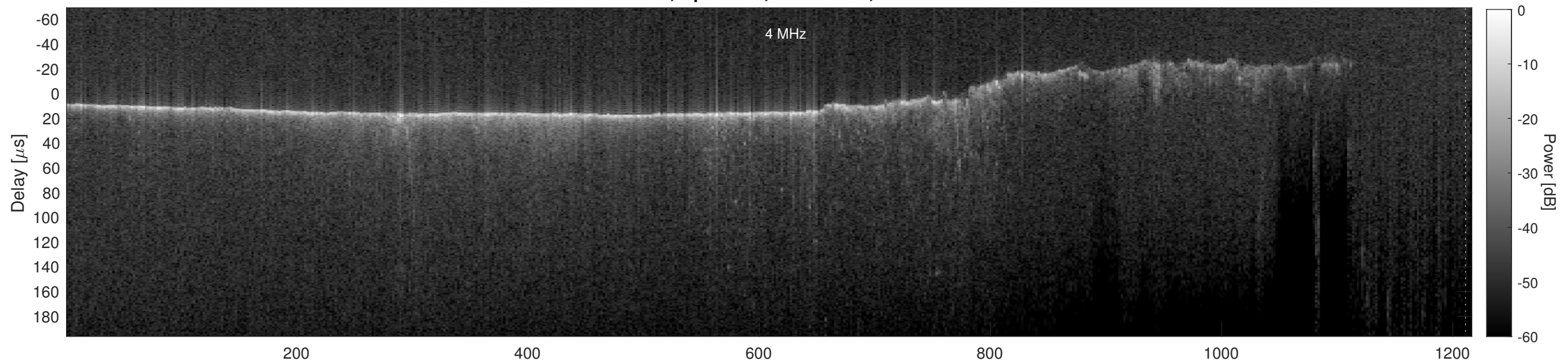
Orbit 11444, Cluttergram
