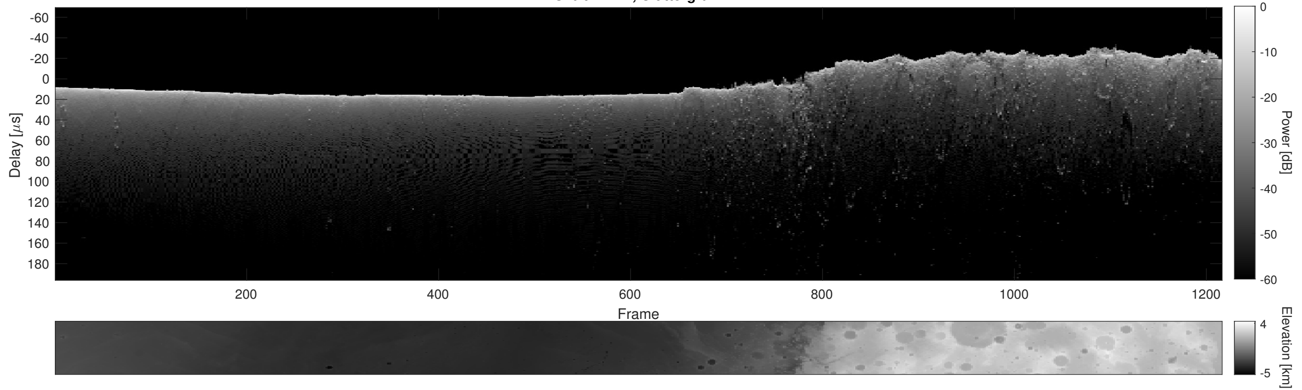
Orbit 11444, Cluttergram
