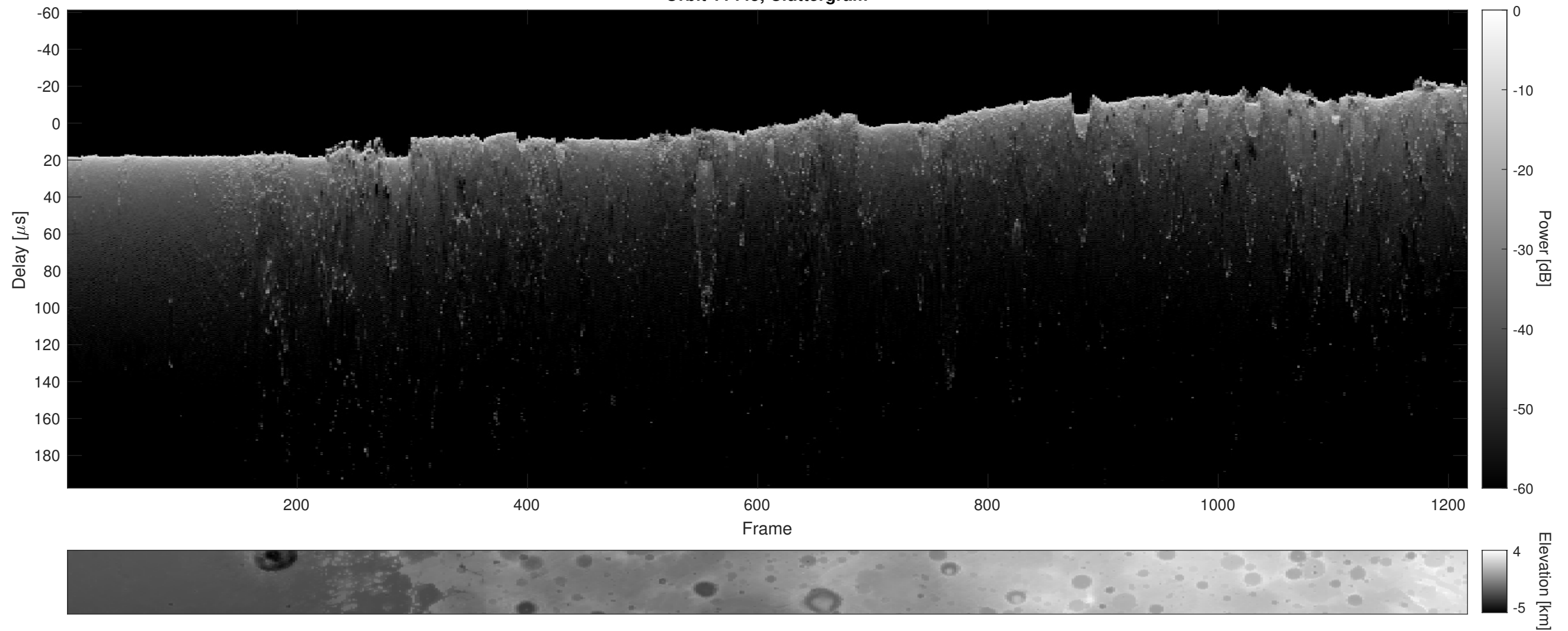
Orbit 11445, Cluttergram
