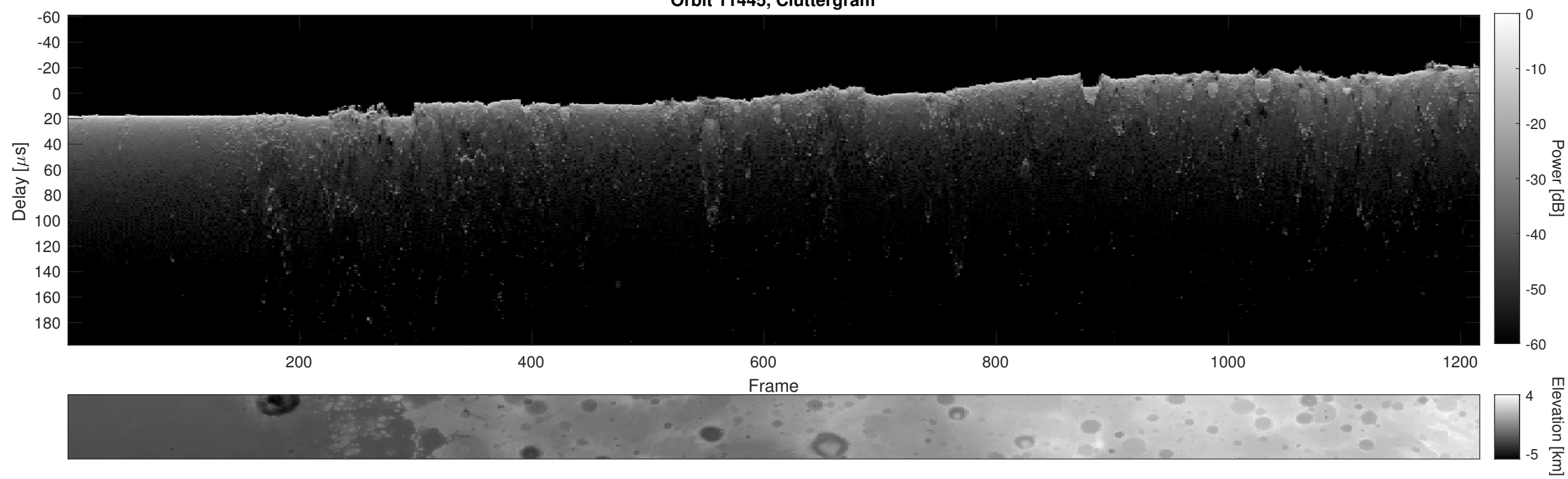
Orbit 11445, Cluttergram
