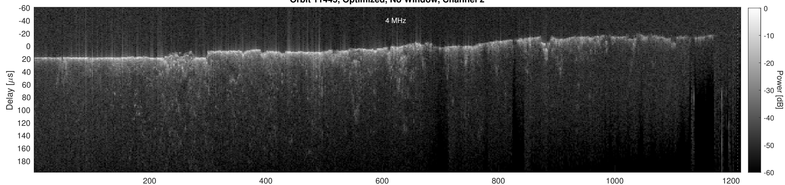
Orbit 11445, Cluttergram
