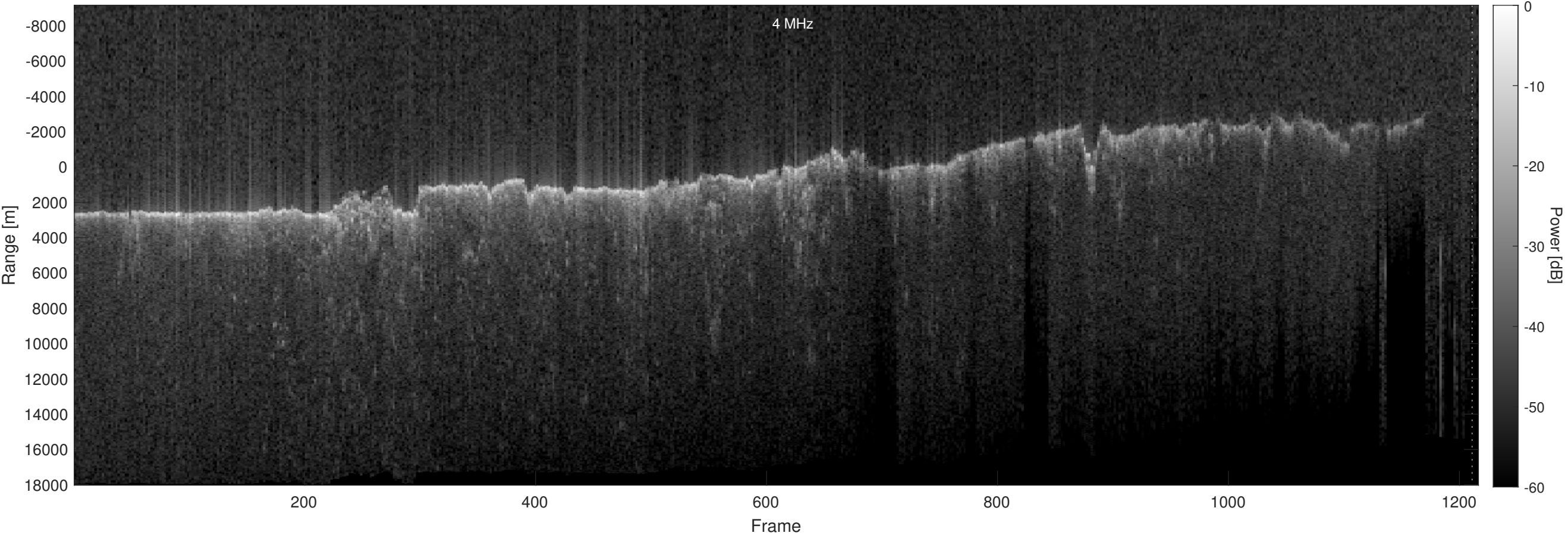
Orbit 11445, Optimized, No Window, Depth-Corrected, Channel 2
