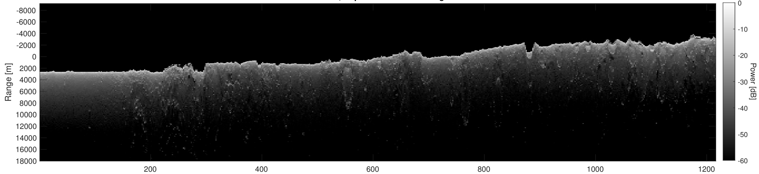
Orbit 11445, Depth-Corrected Cluttergram
