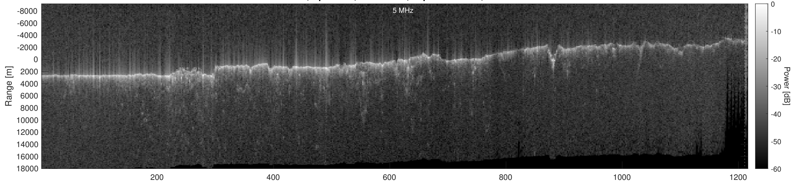
Orbit 11445, Optimized, No Window, Depth-Corrected, Channel 2
