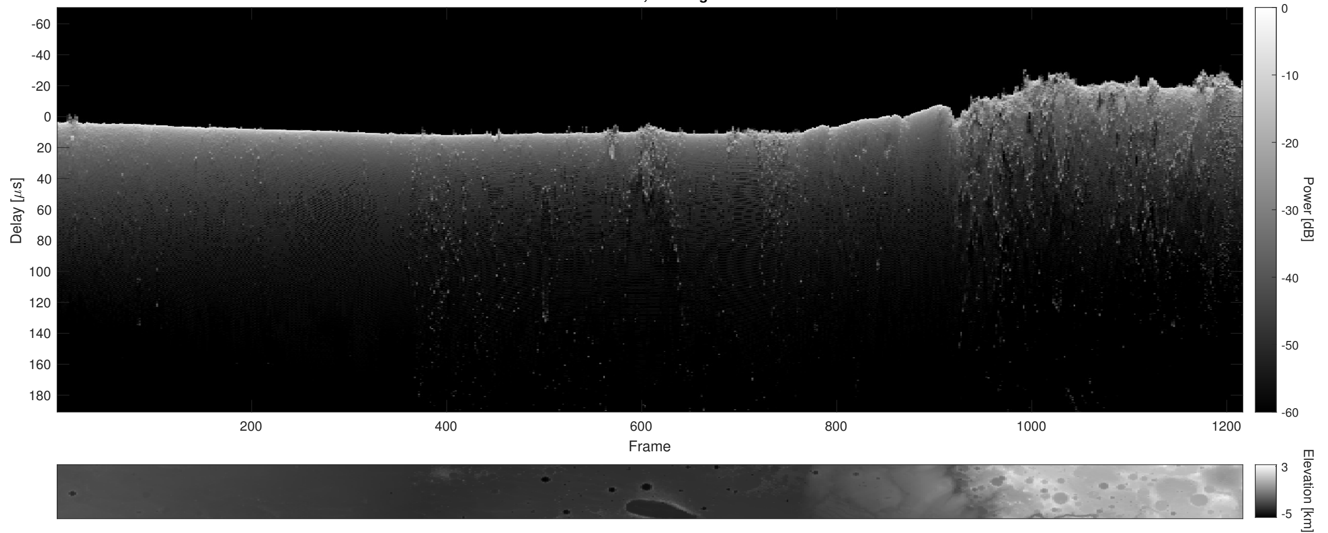
Orbit 11447, Cluttergram
