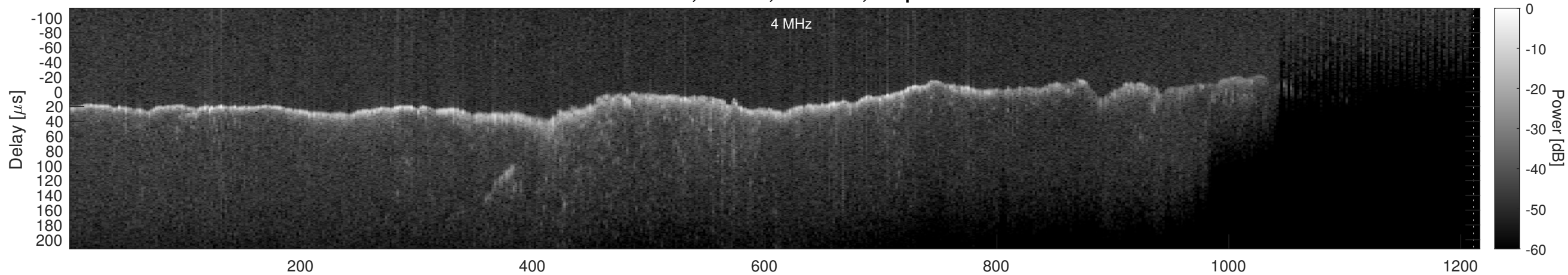
Orbit 11448, Window, Channel 2, Optimized
