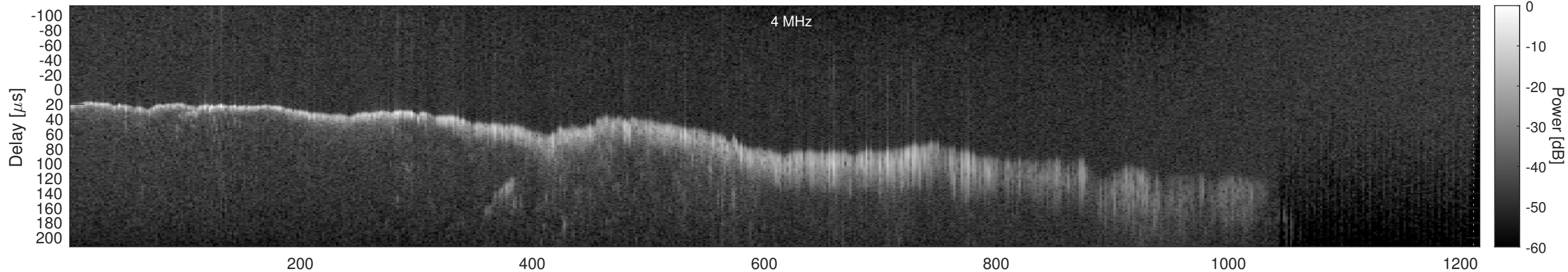
Orbit 11448, Window, Channel 2, Chapman
