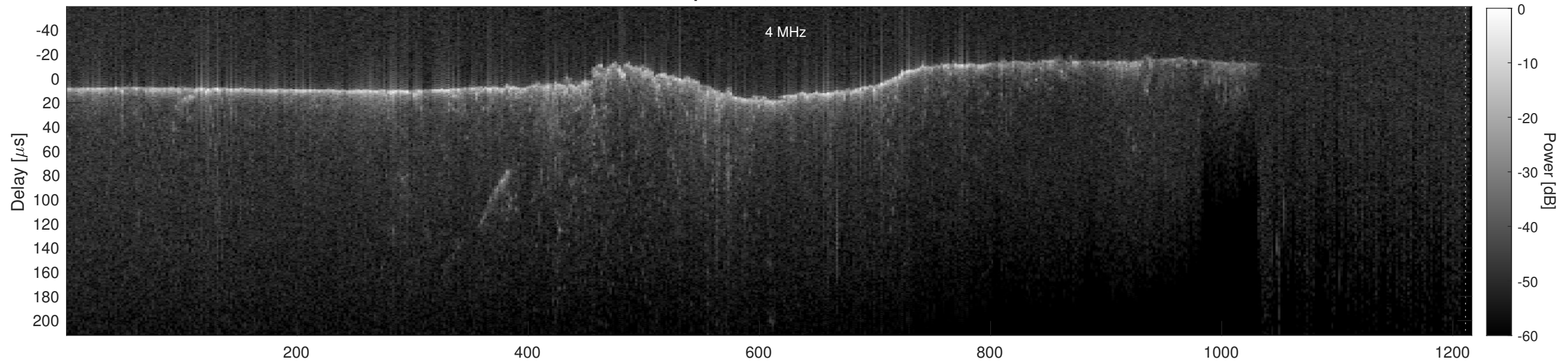
Orbit 11448, Cluttergram
