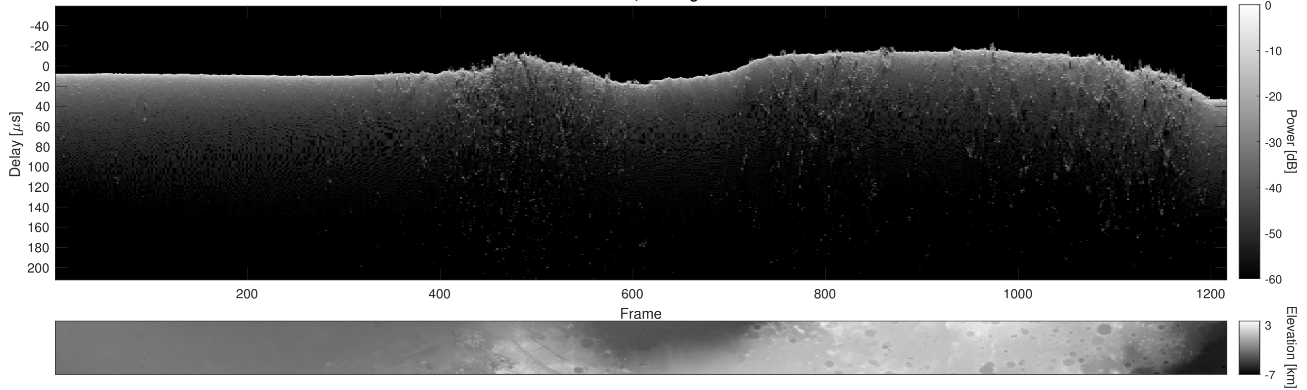
Orbit 11448, Cluttergram
