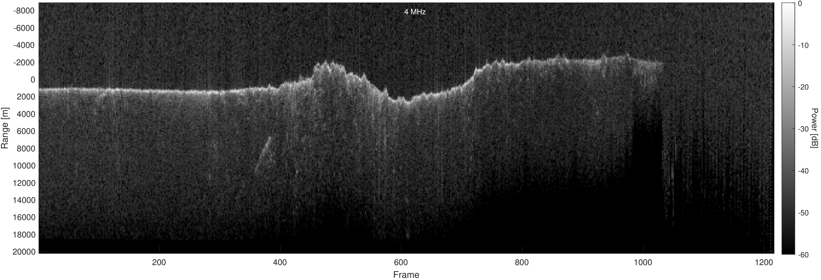
Orbit 11448, Optimized, Window, Depth-Corrected, Channel 2
