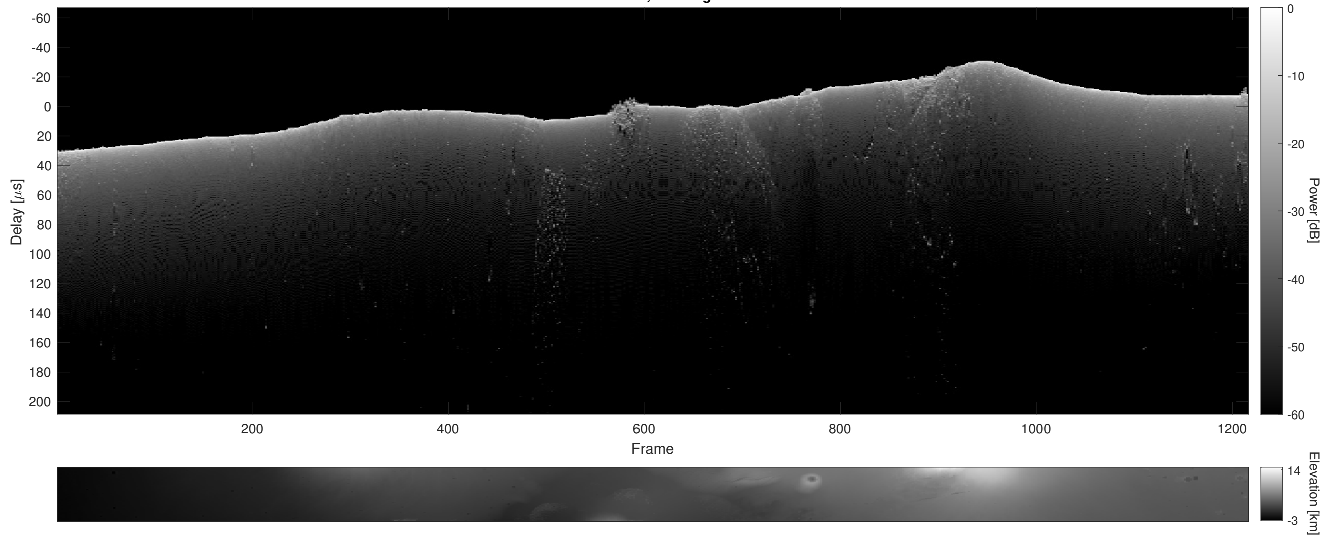
Orbit 11450, Cluttergram
