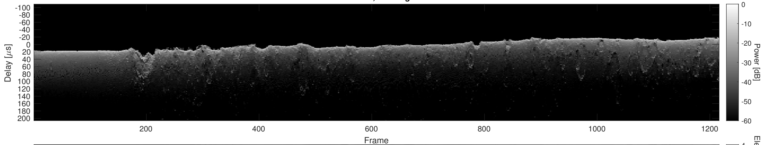
Orbit 11452, Cluttergram
