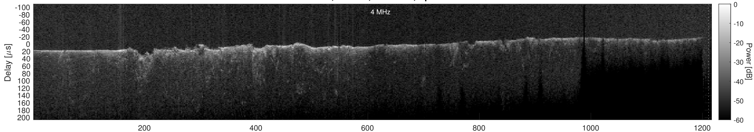
Orbit 11452, Cluttergram
