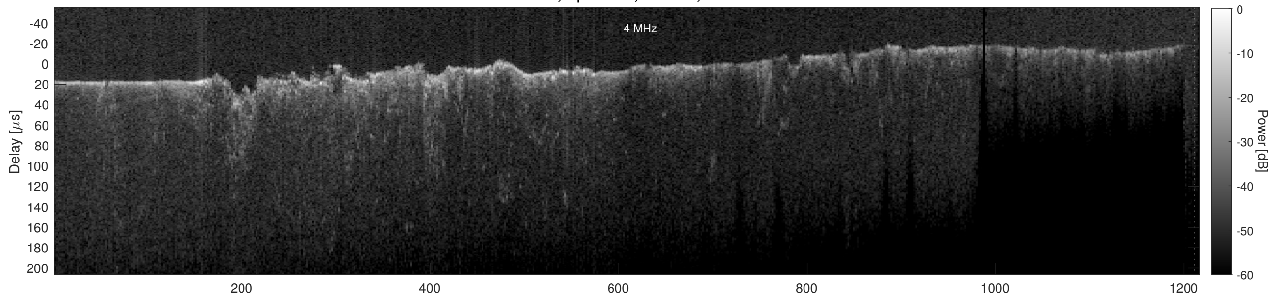
Orbit 11452, Cluttergram
