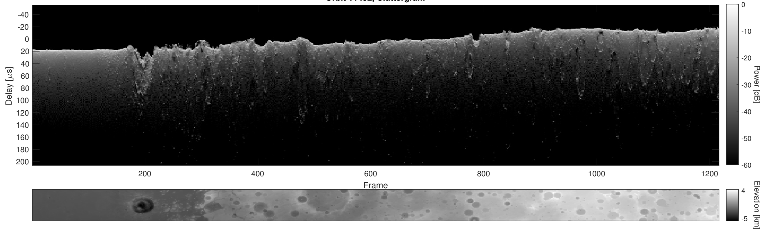
Orbit 11452, Cluttergram
