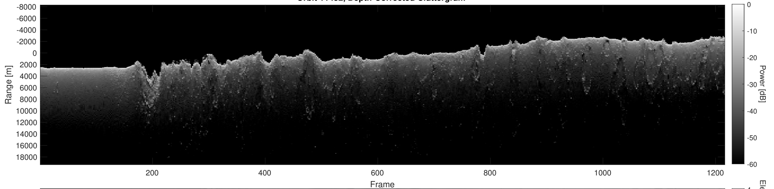
Orbit 11452, Depth-Corrected Cluttergram
