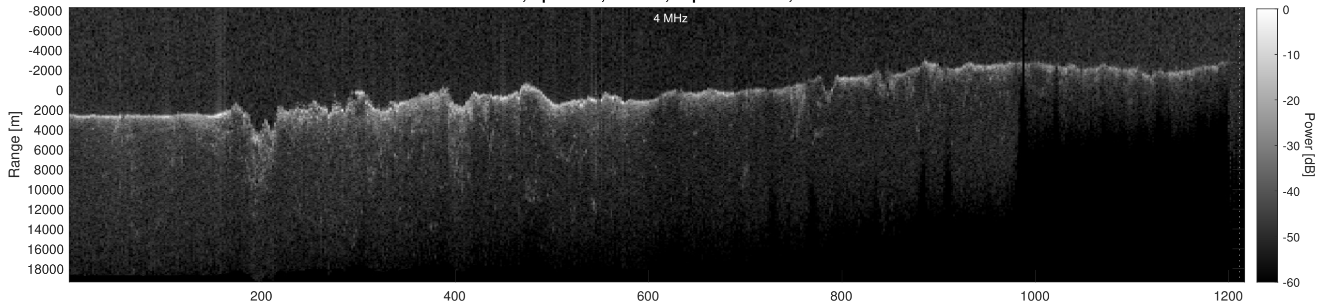
Orbit 11452, Depth-Corrected Cluttergram
