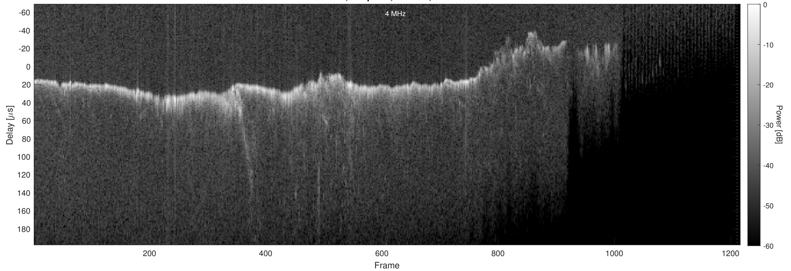
Orbit 11455, Chapman, Window, Channel 2
