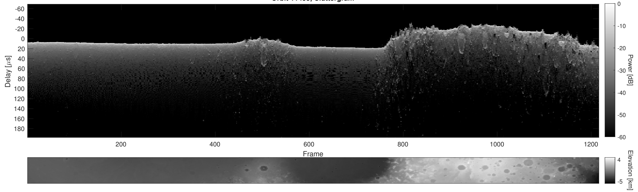
Orbit 11455, Cluttergram
