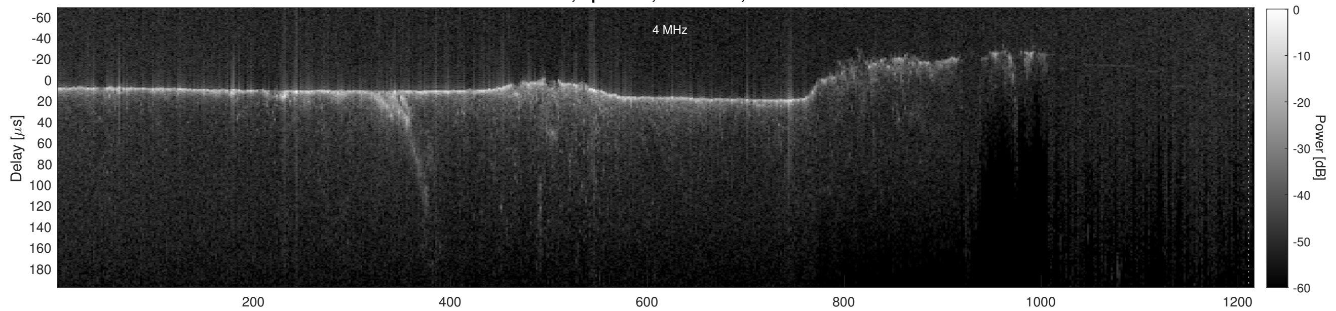
Orbit 11455, Cluttergram
