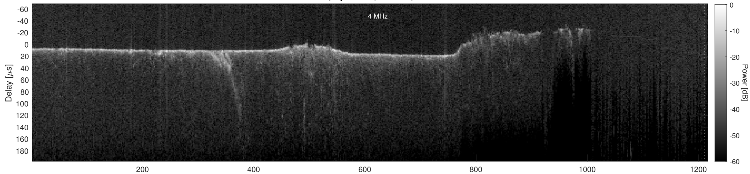
Orbit 11455, Cluttergram
