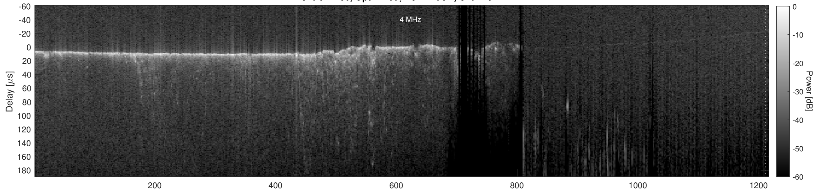
Orbit 11456, Cluttergram
