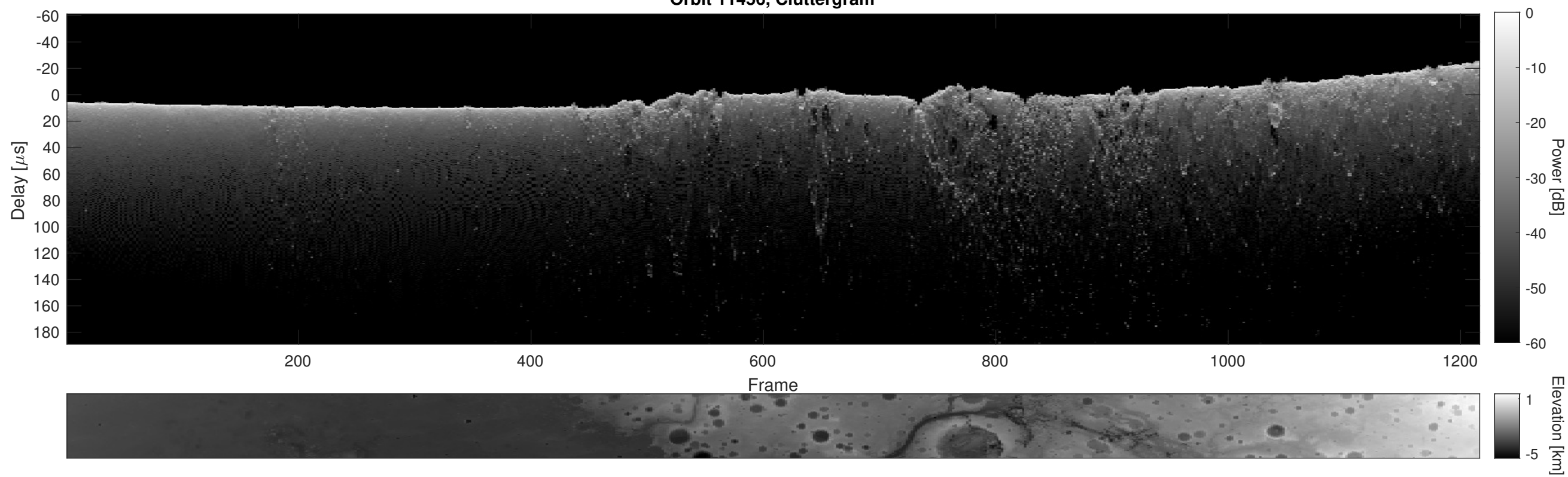
Orbit 11456, Cluttergram
