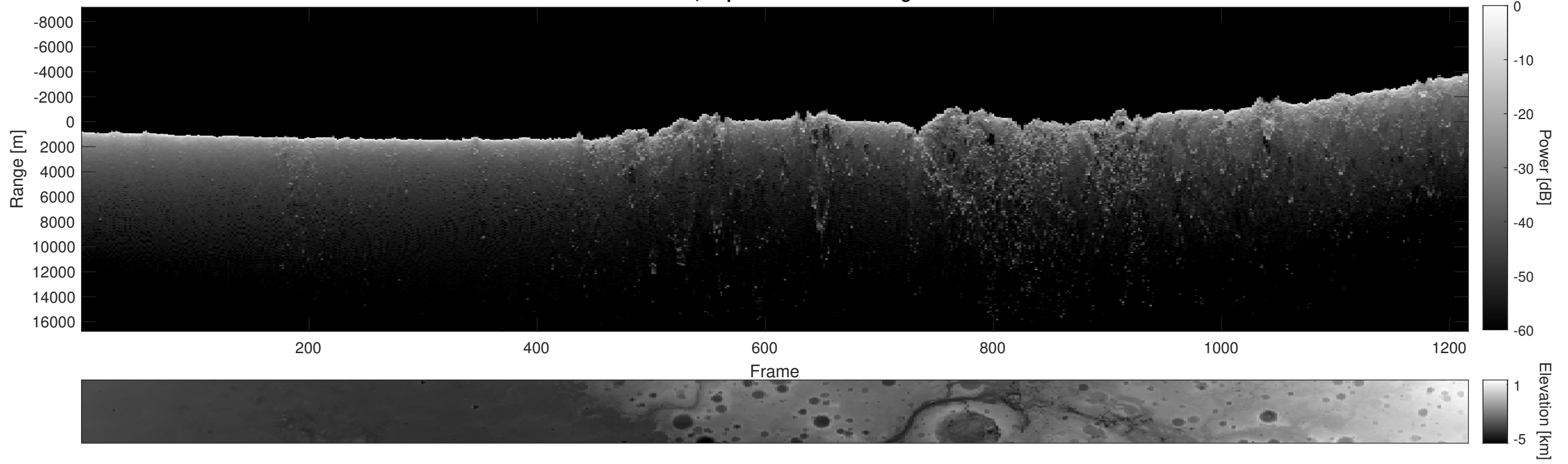
Orbit 11456, Depth-Corrected Cluttergram
