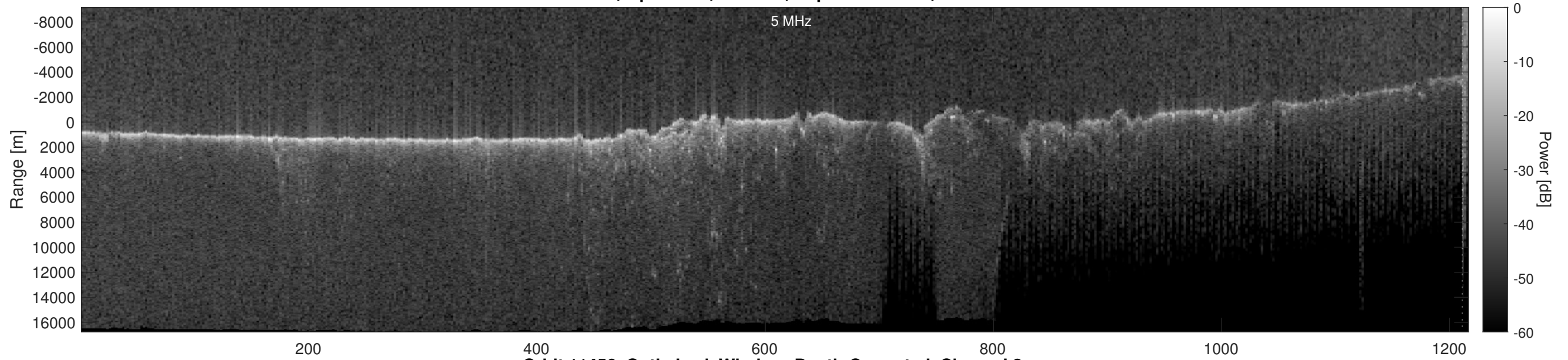
Orbit 11456, Optimized, Window, Depth-Corrected, Channel 2
