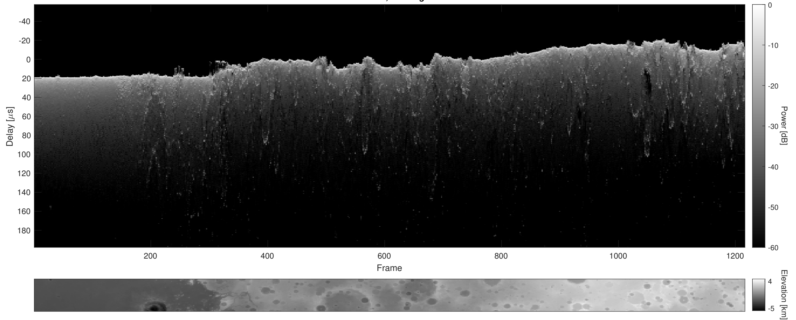
Orbit 11459, Cluttergram
