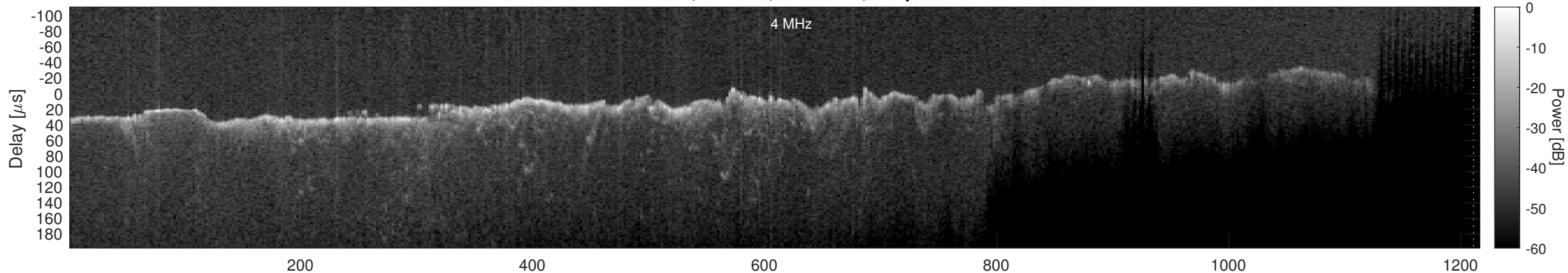
Orbit 11459, Window, Channel 2, Optimized
