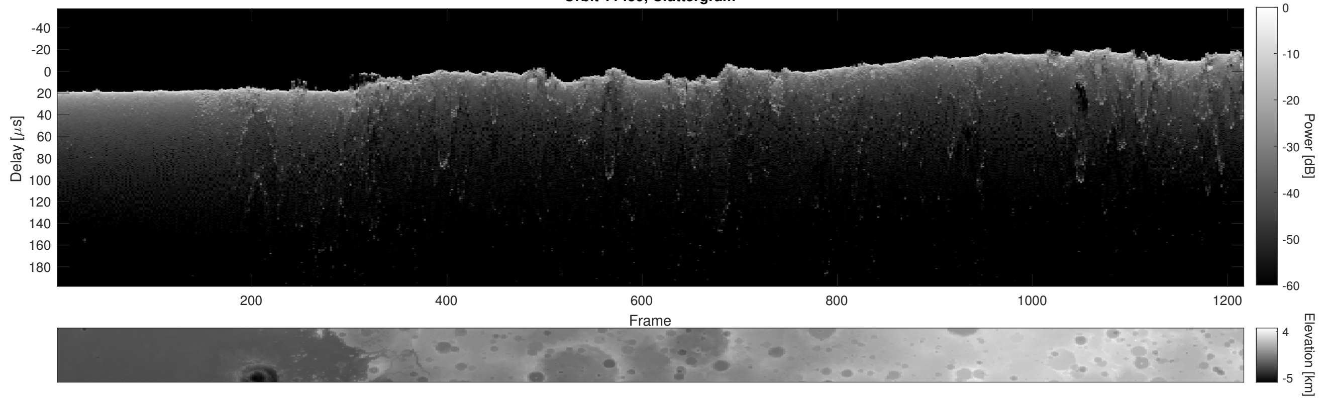
Orbit 11459, Cluttergram
