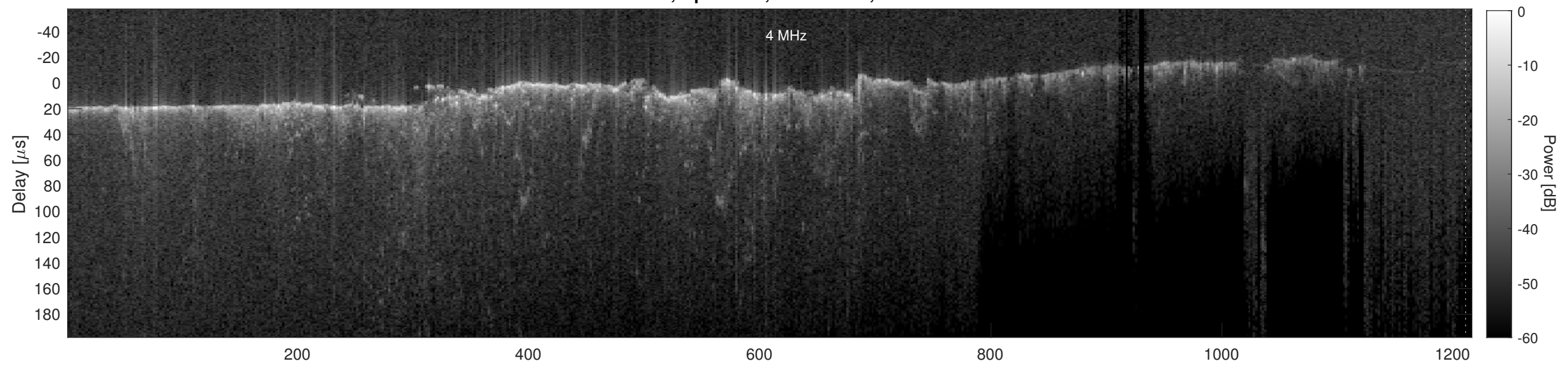
Orbit 11459, Cluttergram
