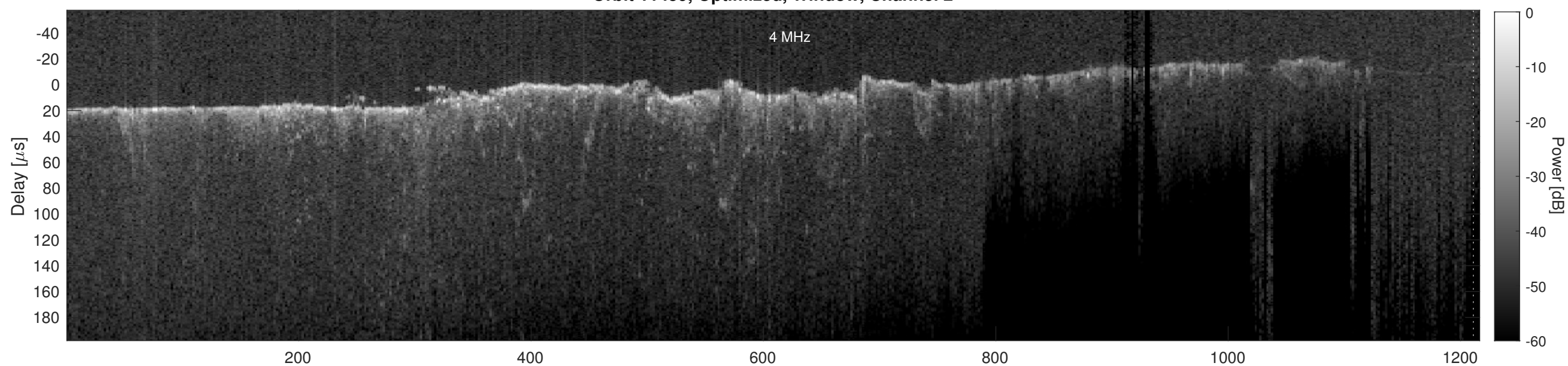
Orbit 11459, Cluttergram
