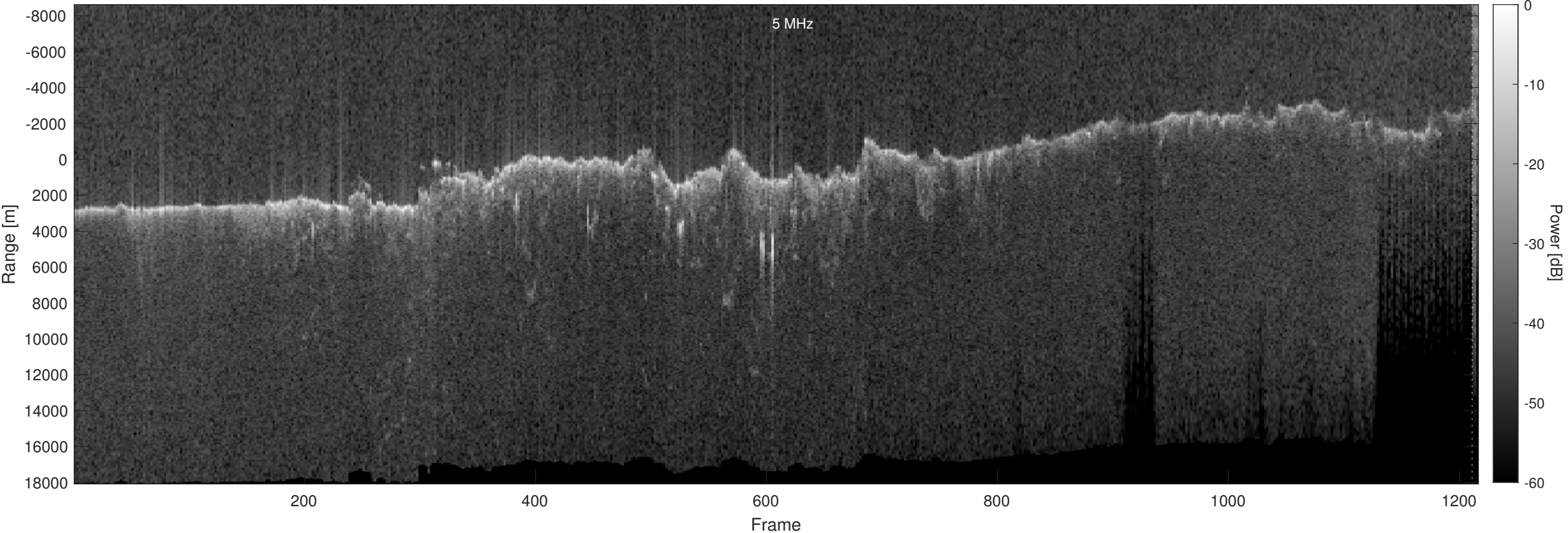
Orbit 11459, Optimized, Window, Depth-Corrected, Channel 2
