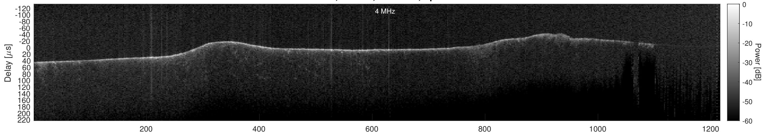
Orbit 11464, Cluttergram
