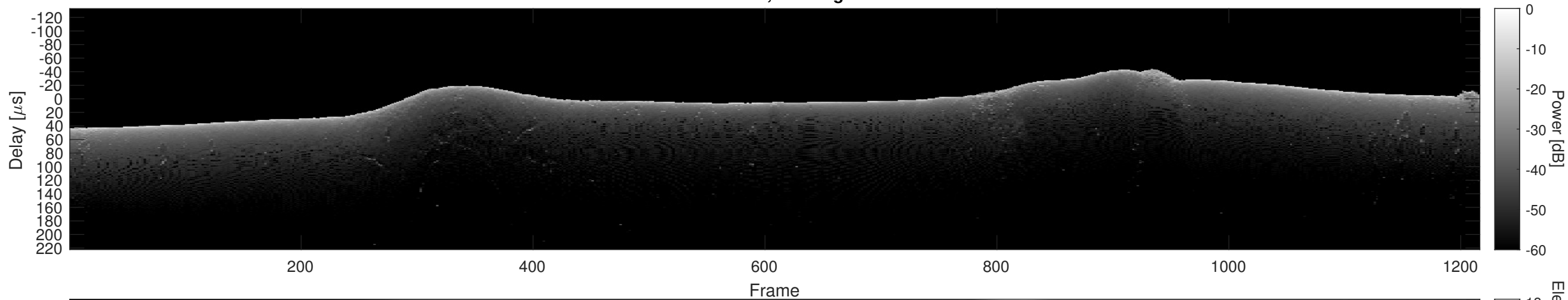
Orbit 11464, Cluttergram
