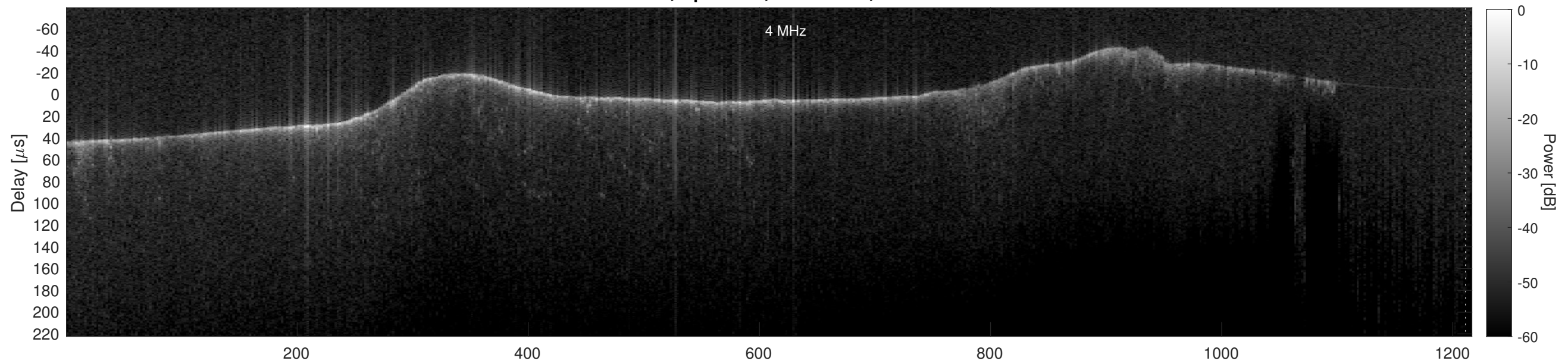
Orbit 11464, Cluttergram
