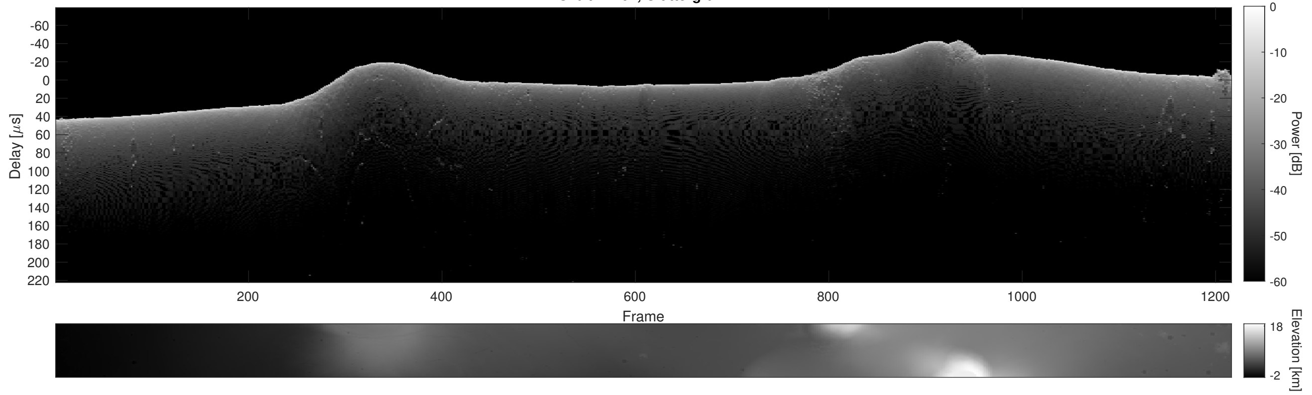
Orbit 11464, Cluttergram
