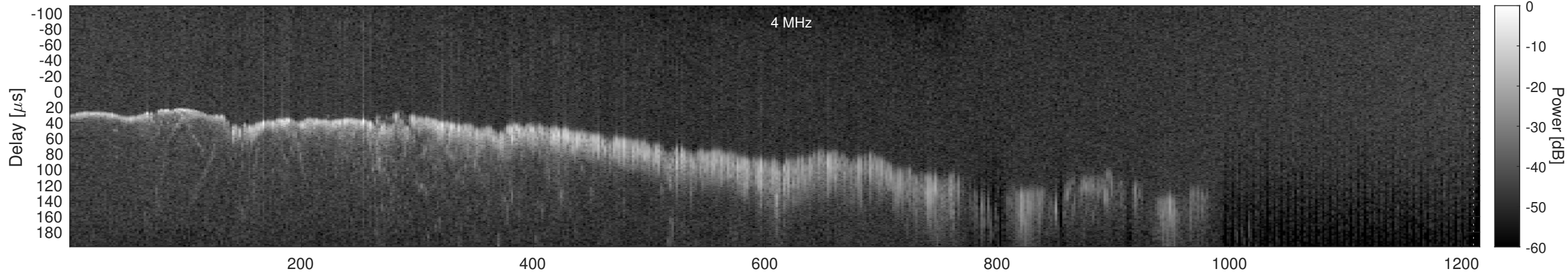
Orbit 11466, Window, Channel 2, Chapman
