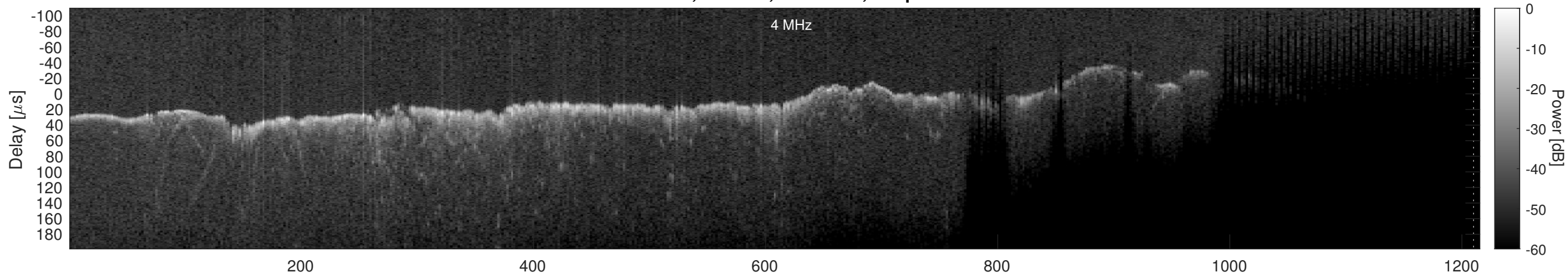
Orbit 11466, Window, Channel 2, Optimized
