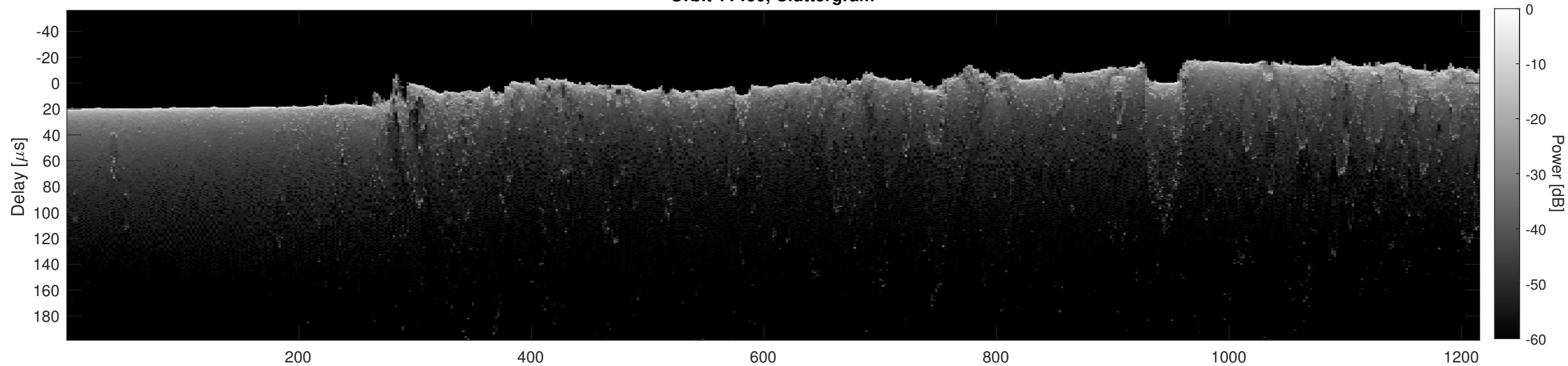
Orbit 11466, Cluttergram
