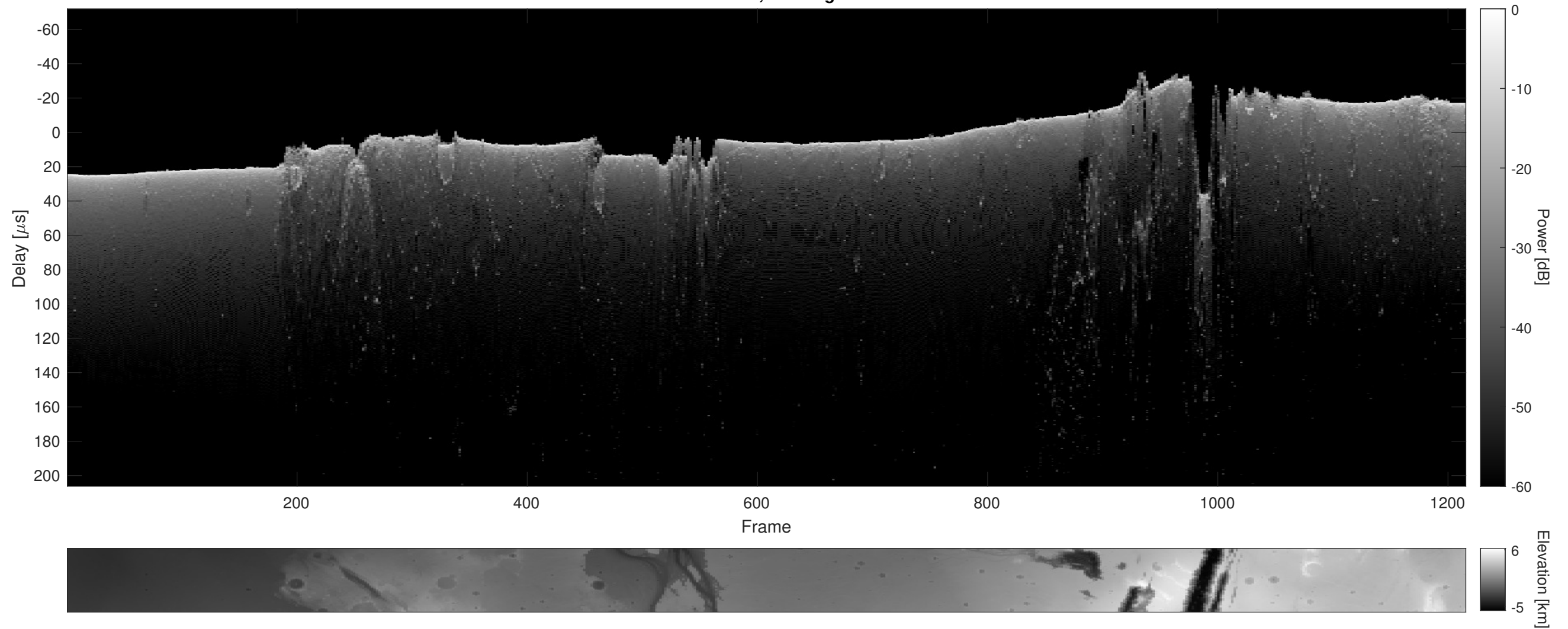
Orbit 11467, Cluttergram
