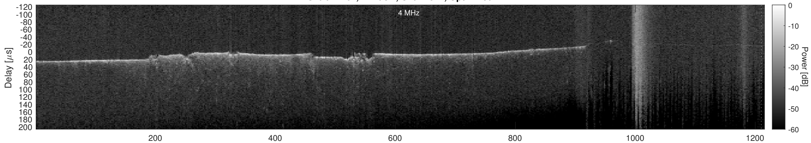
Orbit 11467, Cluttergram
