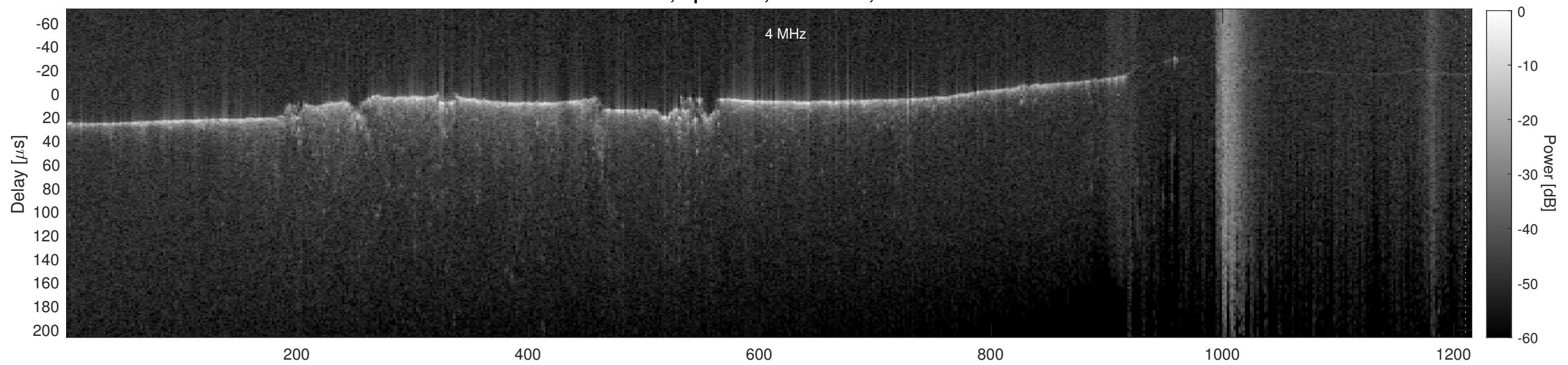
Orbit 11467, Cluttergram
