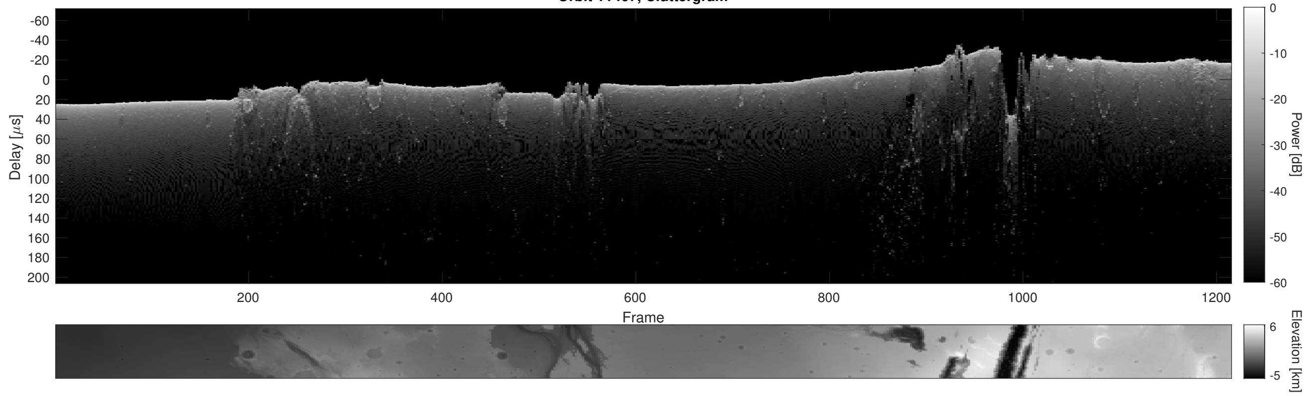
Orbit 11467, Cluttergram
