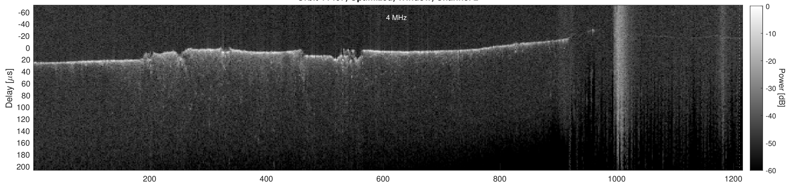
Orbit 11467, Cluttergram
