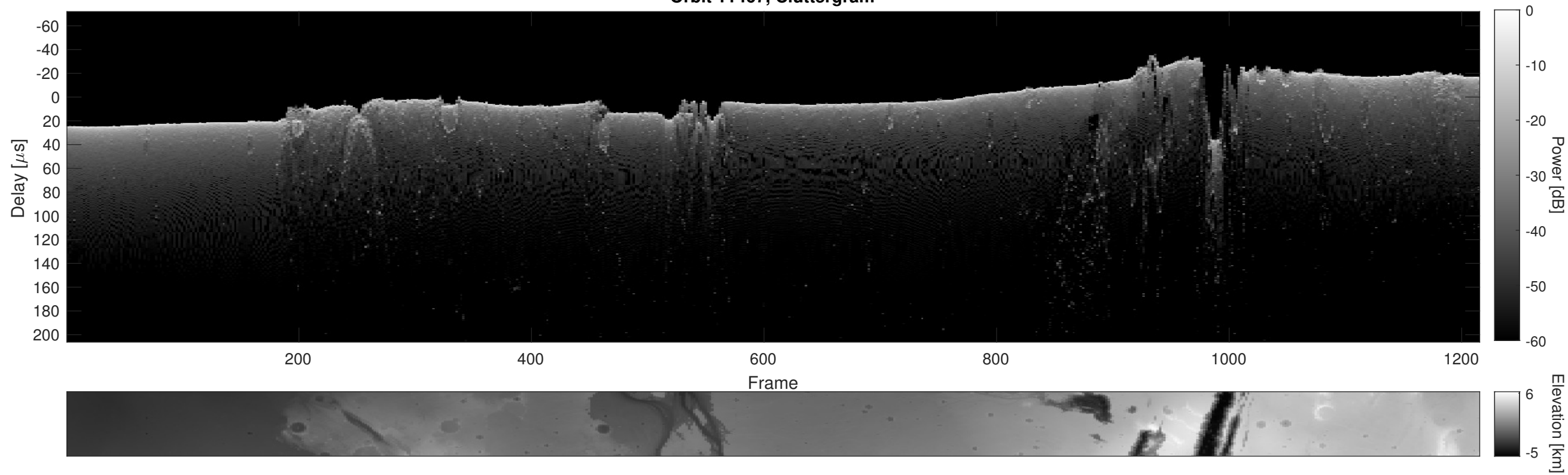
Orbit 11467, Cluttergram
