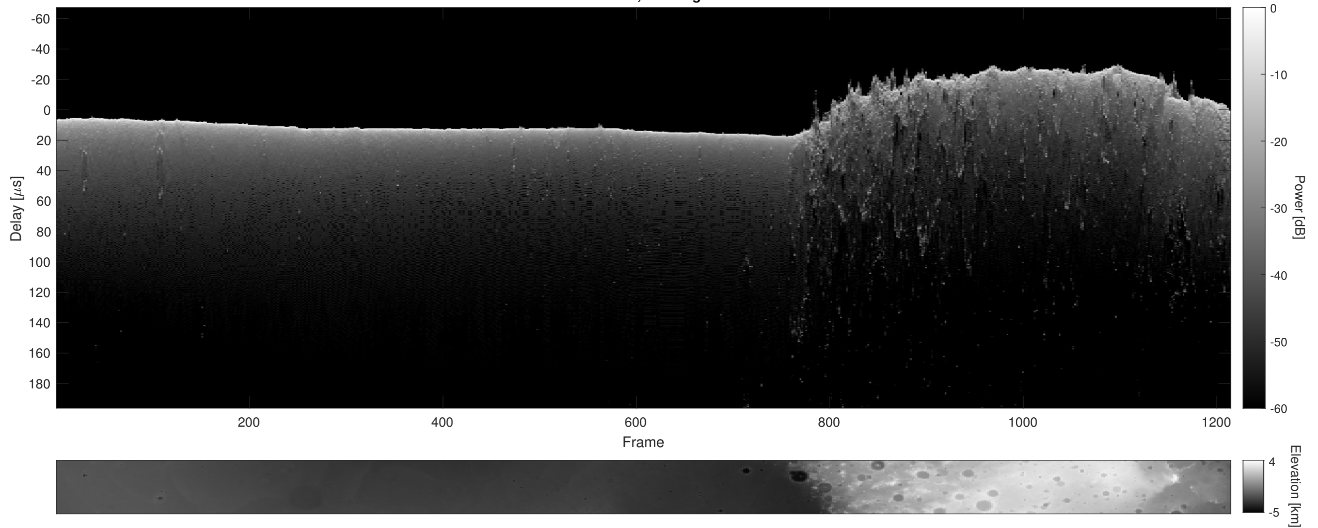
Orbit 11469, Cluttergram
