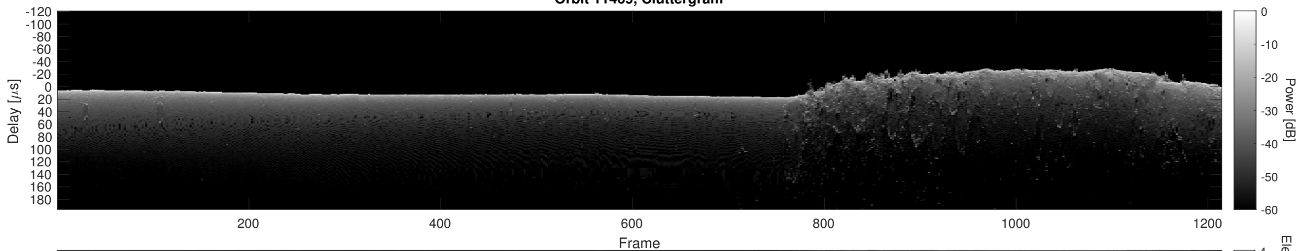
Orbit 11469, Cluttergram
